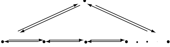
Figure 2: Quiver diagram for the A_{n-1} singularity.
